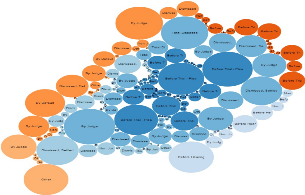
Illustration 13: Bubble Chart
