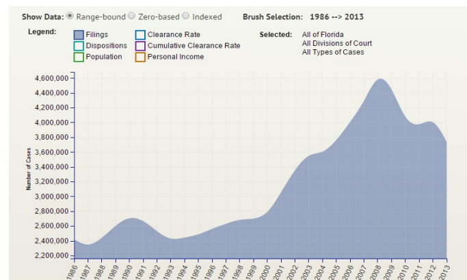
Illustration 3: Filings
