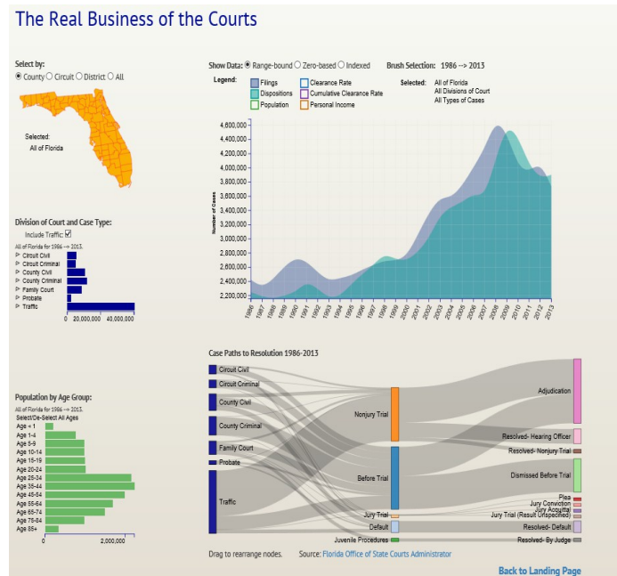
Illustration 2: Discovery Page
