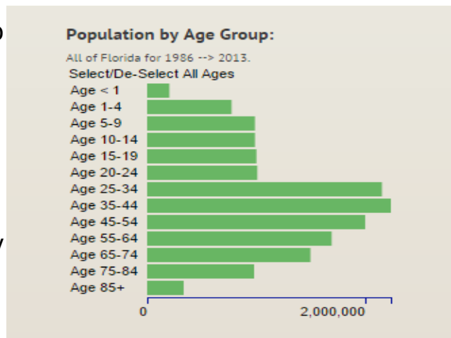
Illustration 8: POP Histogram
