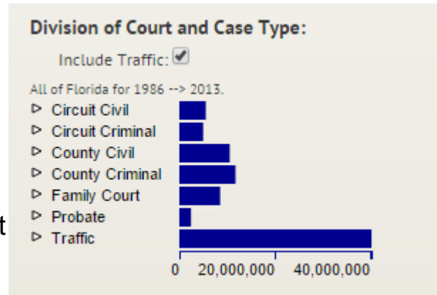
Illustration 6: DOC Histogram
