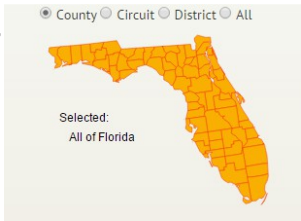
Illustration 9: Map Control
