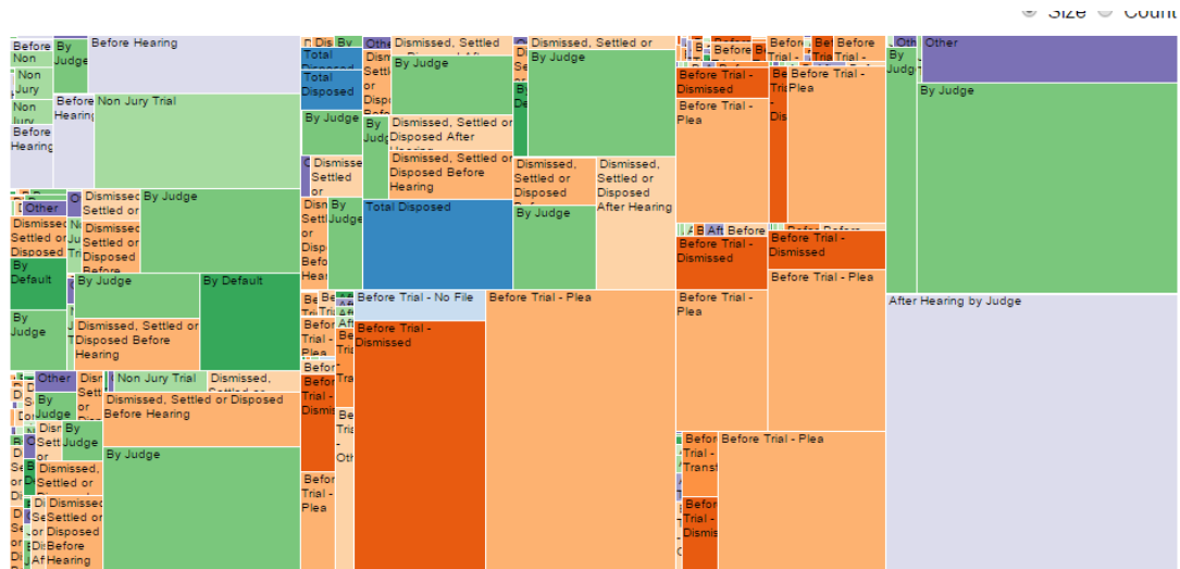
Illustration 15: Treemap
