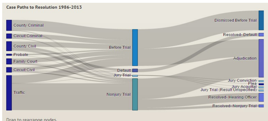
Illustration 10: Sankey Diagram
